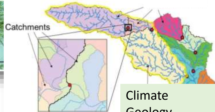
Spatial data
