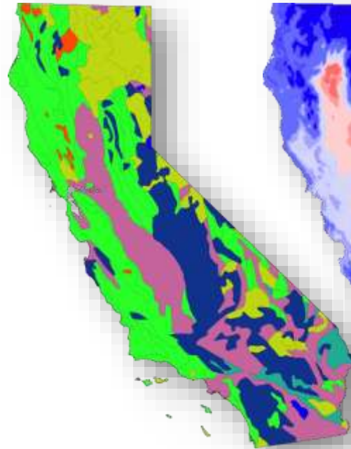
Geology
