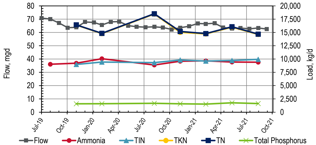
Figure 8-1. Influent: EBDA Monthly Flows and Loads
