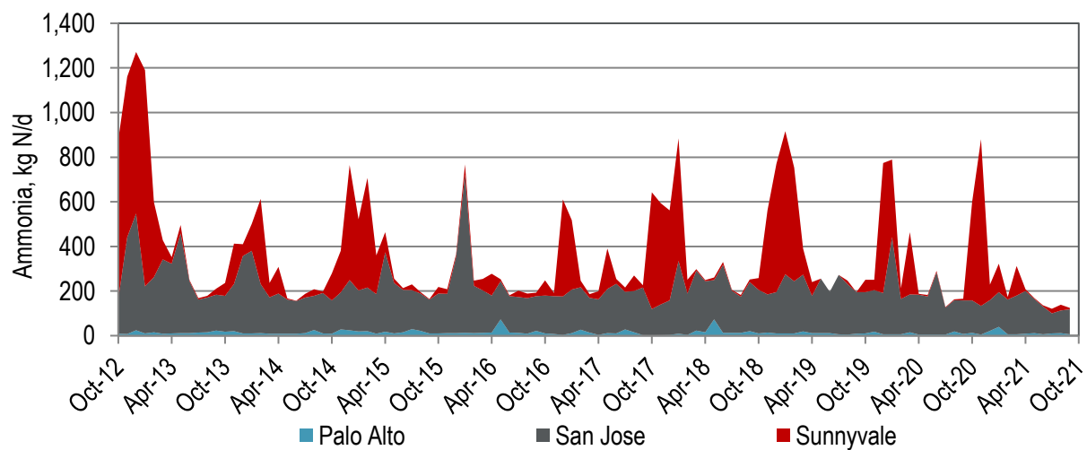
Figure 5-23. Ammonia Load Contribution by Discharger to Lower South Bay
