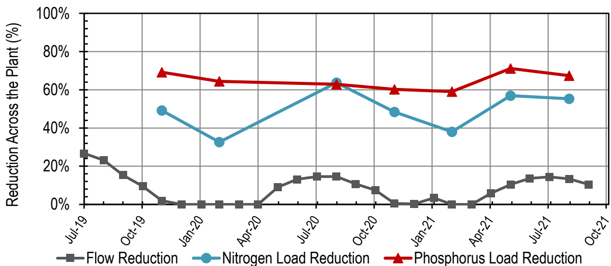
Figure 8-2. Influent: EBDA Monthly Reductions Across the Plant
