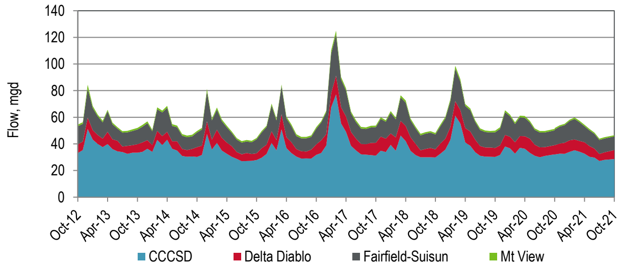
Figure 5-6. Flow Contribution by Discharger to Suisun Bay
