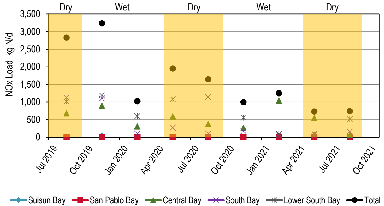
Figure 4-3. Influent: Historical Average Monthly NOx Loads
