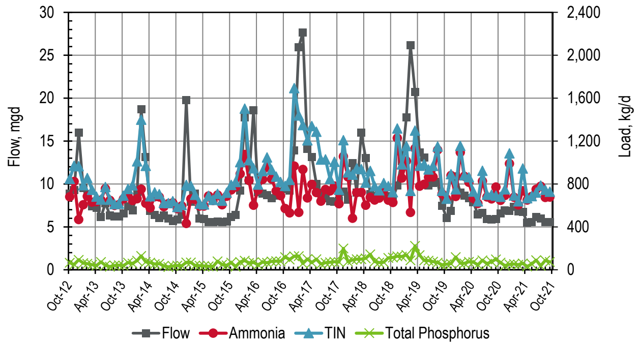
Figure 34-3. Discharge: West County Monthly Flows and Loads
