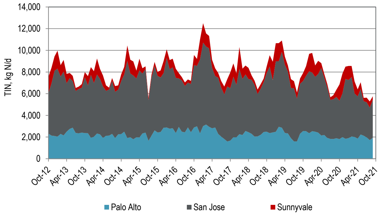
Figure 5-24. TIN Load Contribution by Discharger to Lower South Bay
