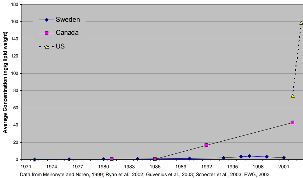
Figure 1-3. Top: concentrations of PBDEs in human breast milk in Sweden; Bottom: the same data, plotted with similar information from Canada and the United States
