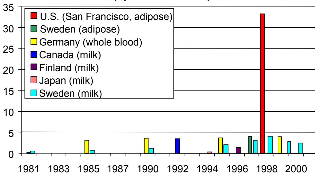
Figure 1-2. PBDEs in human tissues (figure from Kim Hooper, Cal EPA; San Francisco data from She et al., 2002)
