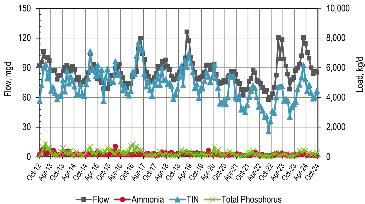
Figure 21-3. Discharge: San Jose Monthly Flows and Loads
